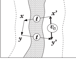
FIG. 2. The external nonlocal “potential” of Eq. (37a) induced in the R region describes new coupling between points x' and y' that takes into account processes in which an electron would tunnel across the barrier, propagate inside the differently ordered electron liquid in the L region, and then tunnel back into R (see text).
