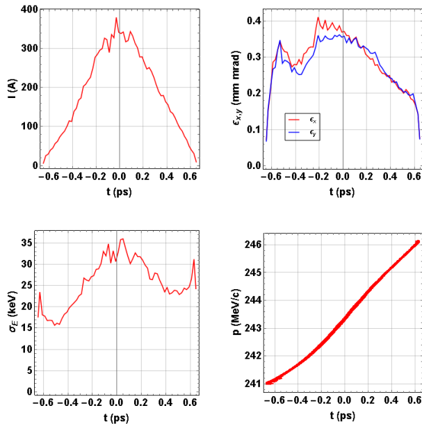
Figure 2: Slice parameters and longitudinal phase space of the optimised S2E bunch at the entrance to the FEL. The normalised emittance meets the spec. of <0.5 mm-mrad and the energy spread is close to the target of 25 keV. The peak of the slice-averaged current is slightly less than 400 A in order to minimise energy chirp, nevertheless the energy chirp of \sim 4 MeV/ps exceeds the spec. of 1 MeV/ps.
