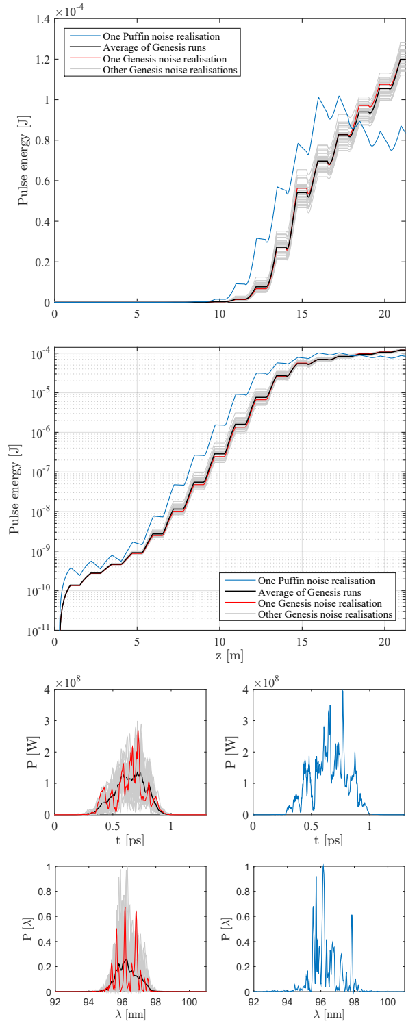
Figure 3: FEL simulation results. Top and second from top: FEL pulse energy with distance through the undulator on linear and log scales. Below: temporal profiles and spectra at saturation (15 m). For each plot there are multiple shot noise realisations shown for the Genesis results (grey), with one typical case highlighted (red) and the average also shown (black). One shot noise realisation is shown for Puffin (blue).
