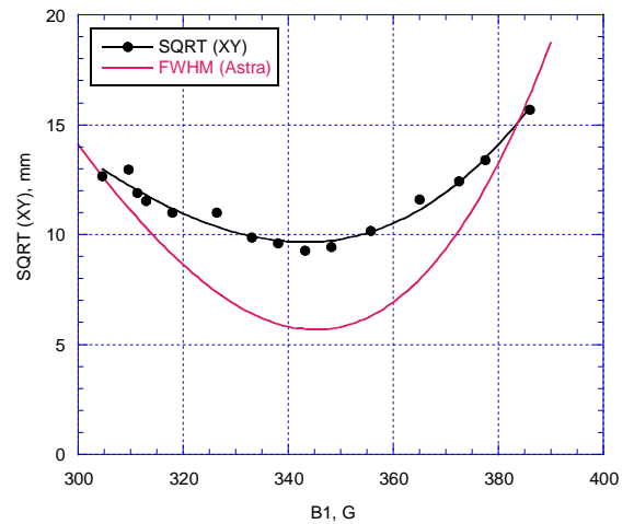
Figure 6: FWHM beam size at a bunch charge of 54 pC as a function of the first solenoid field compared to the results from the ASTRA model.
