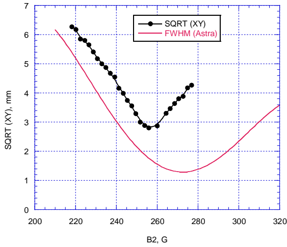
Figure 7: FWHM beam size at a bunch charge of 54 pC as a function of the second solenoid field compared to the results from the ASTRA model.
