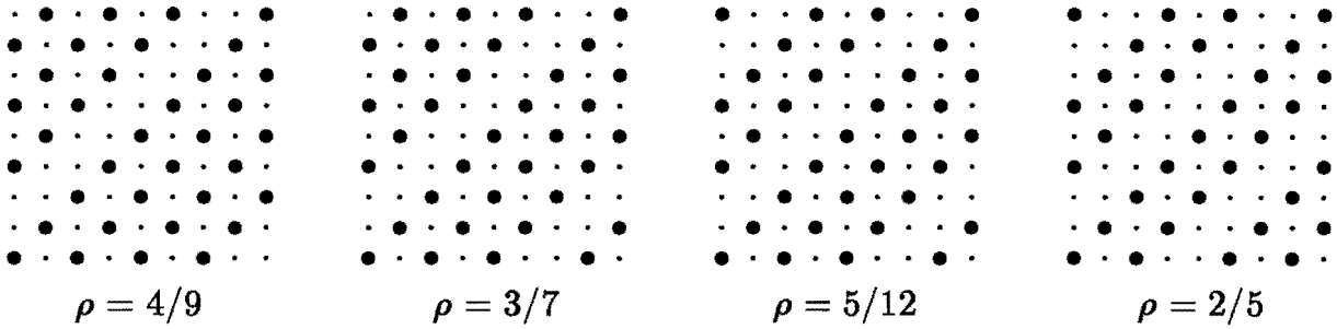
Figure 6: Neutral phases with 1/3 < \rho < 1/2 in the U = 8 restricted phase diagram.
