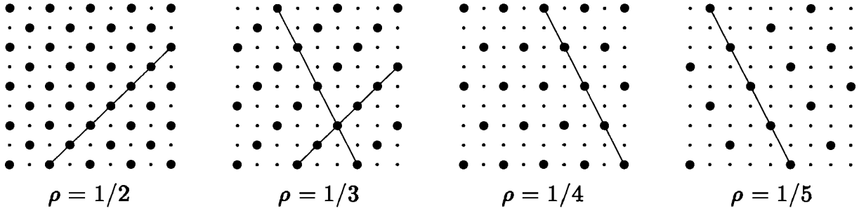
Figure 3: Characteristic configurations derived by Kennedy [15], which are neutral ground states for large U for the given densities. Large dots: occupied sites; small dots: vacant sites. The lines indicate the characteristic slopes discussed in the text.
