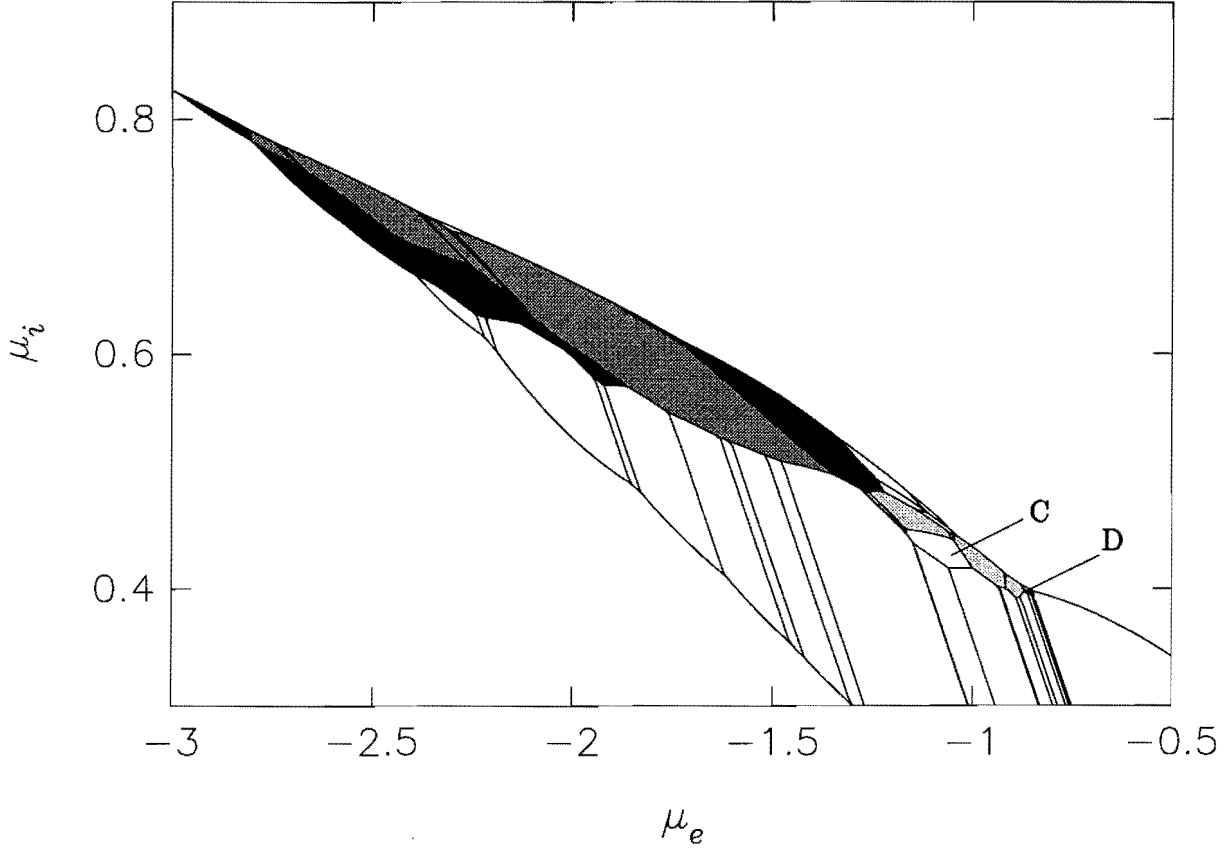
Figure 10: Detail of the restricted phase diagram for U = 2 . Light shading: staggered stripe phases; medium shading: stripe phases; heavy shading: molecular lattices. Phases labelled C and D are discussed in Sec. 3.5.
