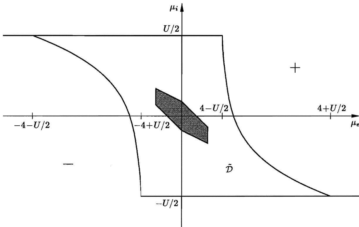
Figure 2: Schematic phase diagram obtained by Gruber et al. [14]. Lines divide the plane of electron ( \mu_e ) and ion ( \mu_i ) chemical potentials into regions (+) and (−) in which the full and empty configurations, respectively, have been proved to be the ground states, and \tilde{D} , in which any translationally non-invariant ground states must be contained. \tilde{D} includes the shaded domain, in which the checkerboard configuration has been shown to be the ground state.
