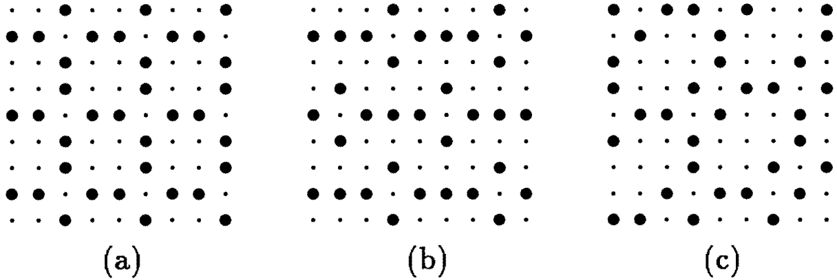
Figure 15: Miscellaneous configurations occurring in the restricted phase diagrams: (a) for U = 6 ; (b) and (c) for U = 2 .
