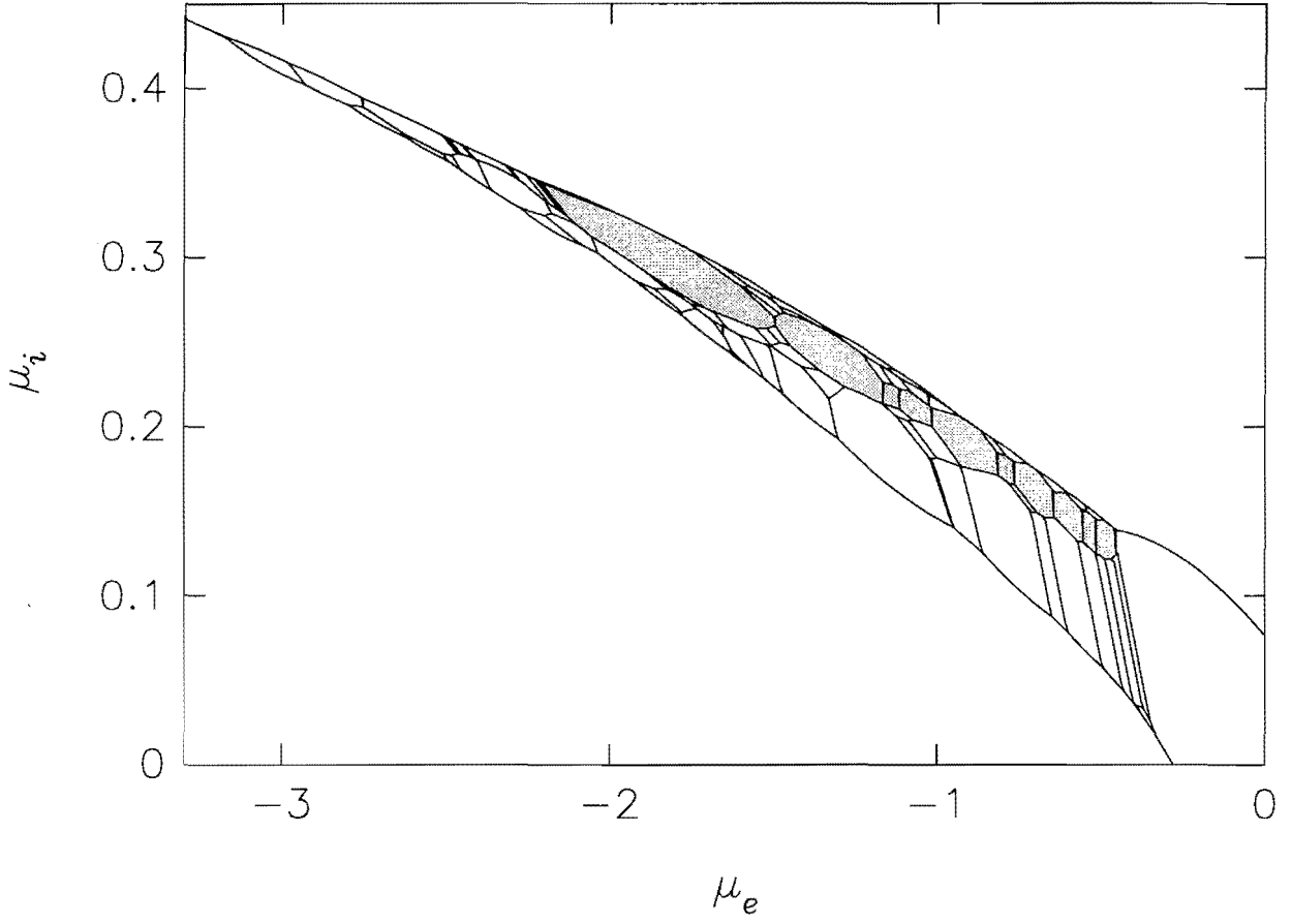
Figure 12: Calculated restricted phase diagram for U = 1 . The shaded areas correspond to the staggered stripe phases (Sec. 3.4).
