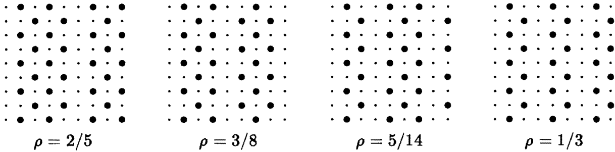
Figure 7: The sequence of neutral ground states in the U = 1 restricted phase diagram.
