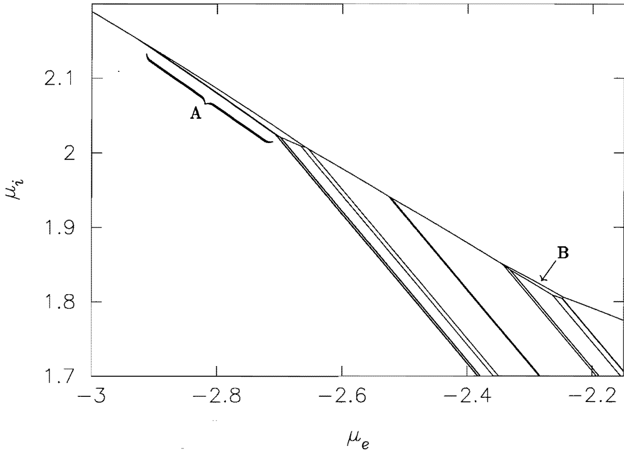
Figure 8: Detail of the calculated restricted phase diagram for U = 6 . Domains labelled A correspond to the stripe configurations (Sec. 3.3), and B points to an unusual insulating phase discussed in Sec. 3.5.
