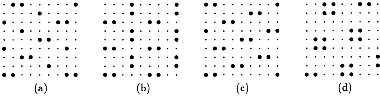
Figure 11: Selected molecular lattices occurring in the U = 2 phase diagram.
