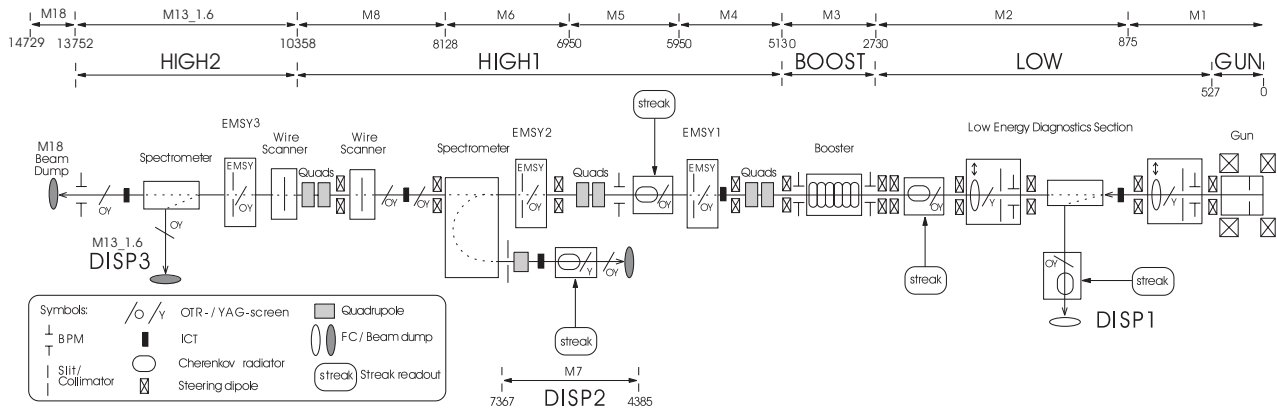
Figure 1: PITZ layout as in 2008/2009. The electron beam propagates from right to left.
