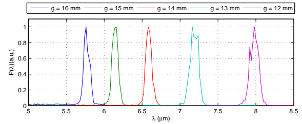
Figure 3: ALICE FEL spectra at different undulator gaps.
