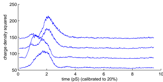
Figure 4: Examples of shot-to-shot bunch profile measurements at the ALICE IR-FEL location obtained with the electro-optic diagnostic.
