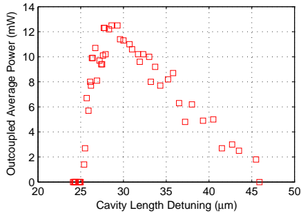
Figure 2: ALICE IR-FEL detuning curve. FEL average power as a function of FEL cavity length detuning.
