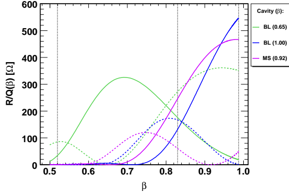
Figure 4: (R/Q)(\beta) plot of the TM_{010,4/5\pi} (dashed) and TM_{010,\pi} (solid) modes. The entrance, transition, and output energy is indicated with vertical dotted lines.
