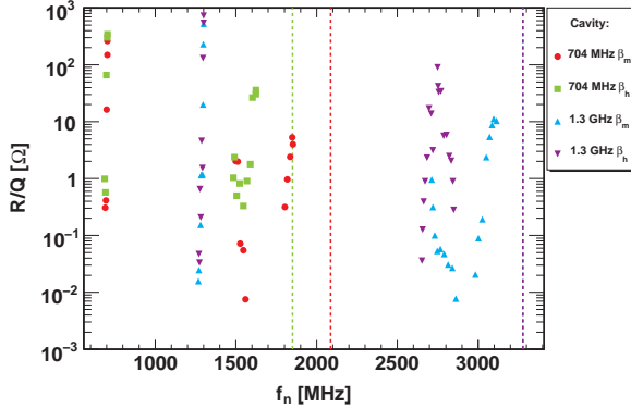
Figure 2: (R/Q)_{\max} of the first three monopole bands. The dashed lines indicate the beam pipe cut-off frequency.
