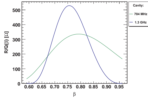
Figure 1: (R/Q)(\beta) plot of the TM_{010,\pi} mode in a 5 cell 704 MHz and a 9 cell 1.3 GHz cavity. The cavities have the same \beta_g=0.74 .
