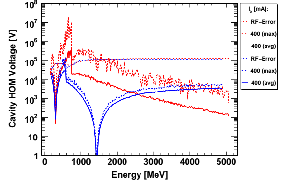
Figure 5: Average (solid) and maximum (dashed) cavity HOM voltages over the beam energy in the cavity centre. The maximum RF voltage error is indicated with dotted lines. The upper (red) curves are the BL layout and the lower (blue) the MS layout.
