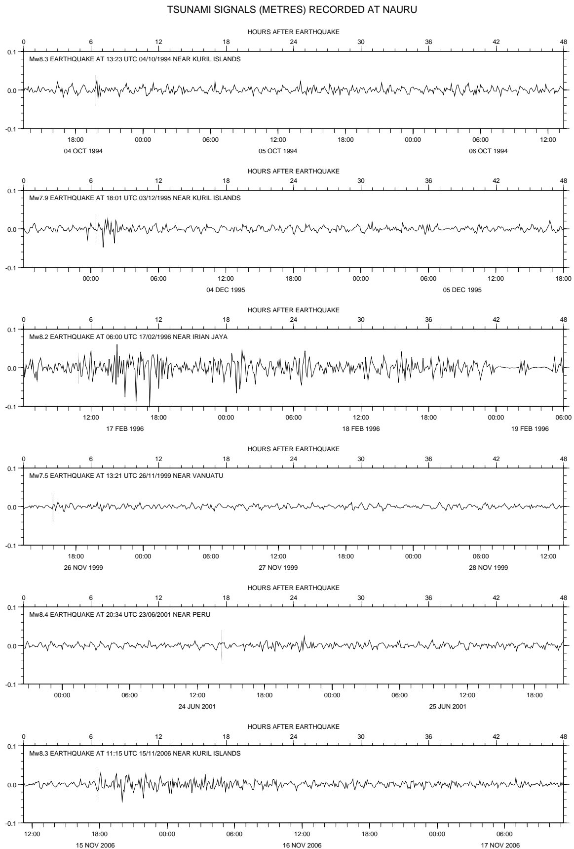
Figure 13a. Tsunami signals (m) recorded by the SEAFRAME at Nauru since installation.
