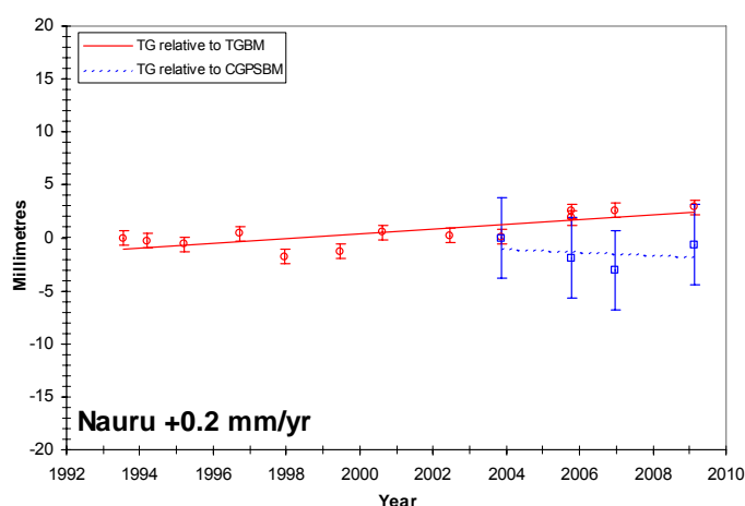
Figure 20. Movement of the SEAFRAME Sensor relative to the Tide Gauge Bench Mark and CGPS station.
