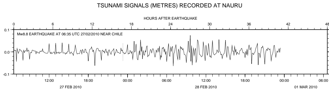
Figure 13b. Tsunami signals (m) recorded by the SEAFRAME at Nauru since installation.
