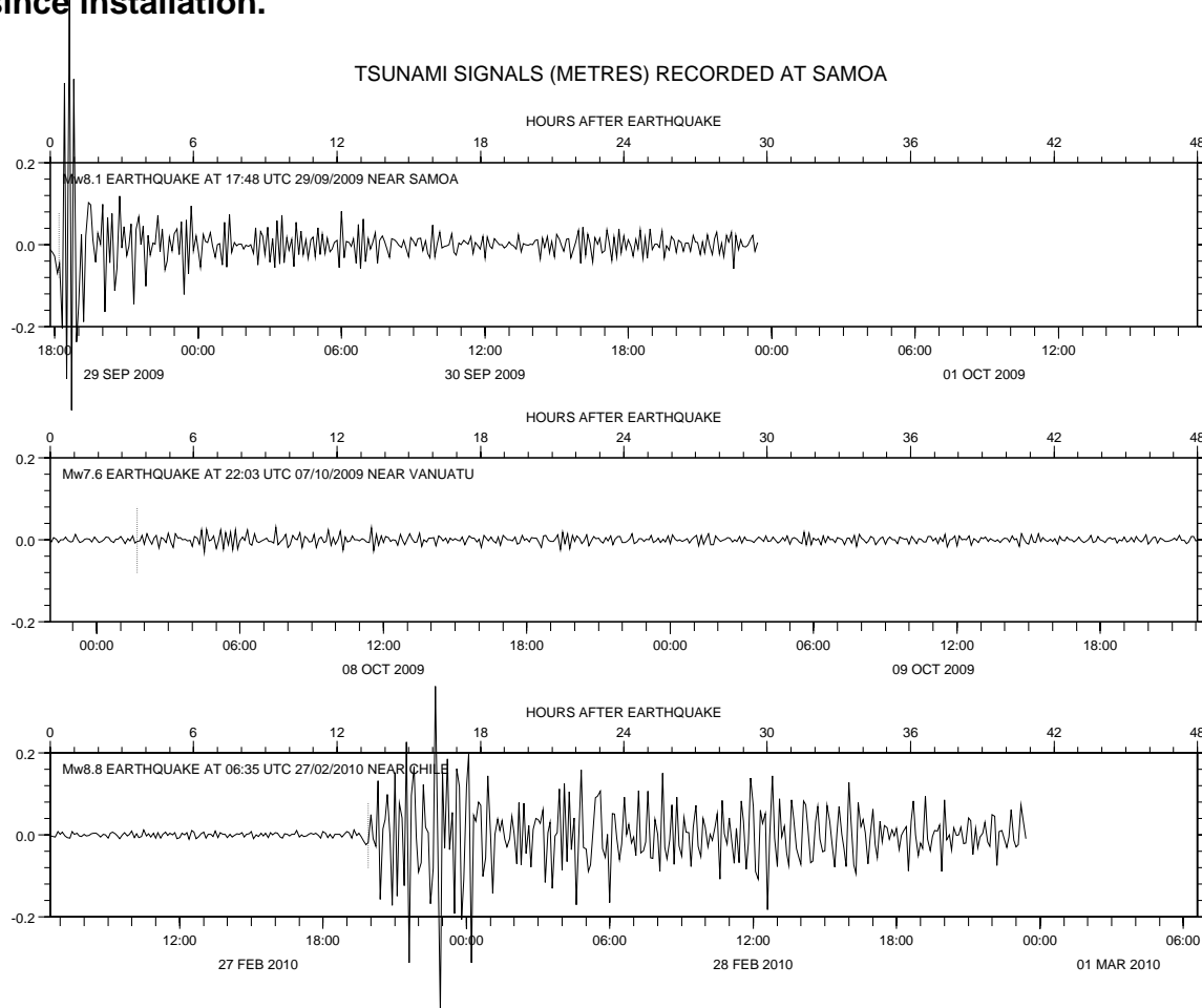
Figure 14d. Tsunami signals (m) recorded by the SEAFRAME at Apia, Samoa since installation.
