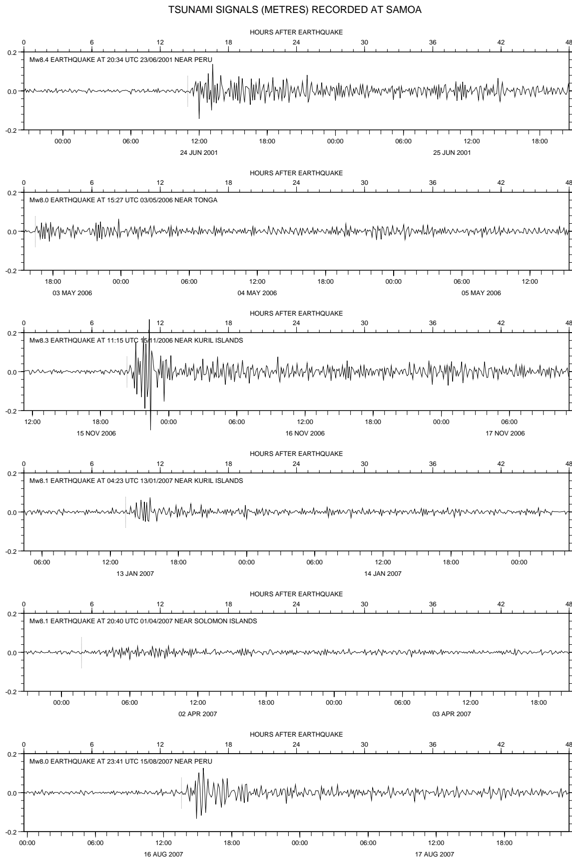
Figure 14c. Tsunami signals (m) recorded by the SEAFRAME at Apia, Samoa since installation.
