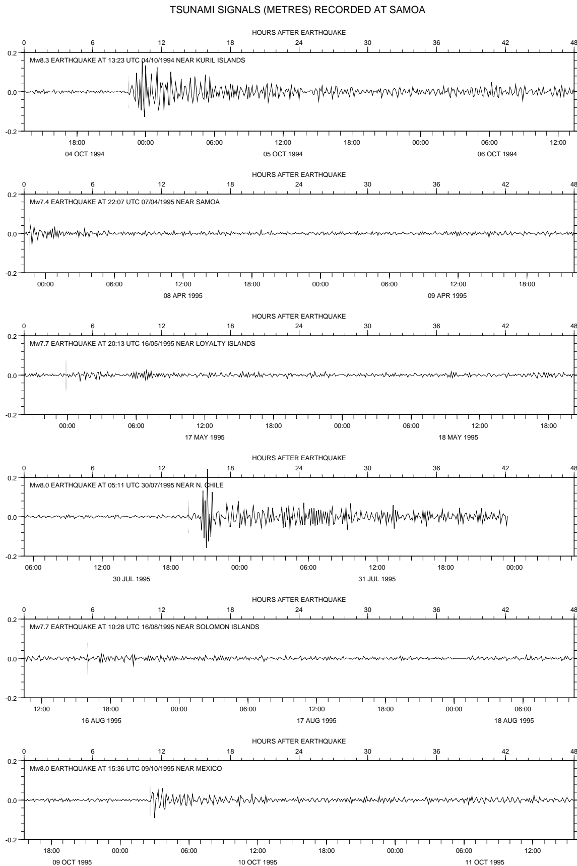
Figure 14a. Tsunami signals (m) recorded by the SEAFRAME at Apia, Samoa since installation.
