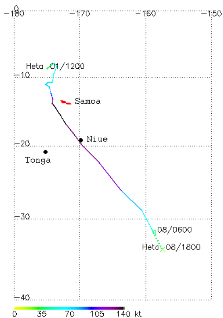
Figure 11. Track of Tropical Cyclone Heta, January 2004
