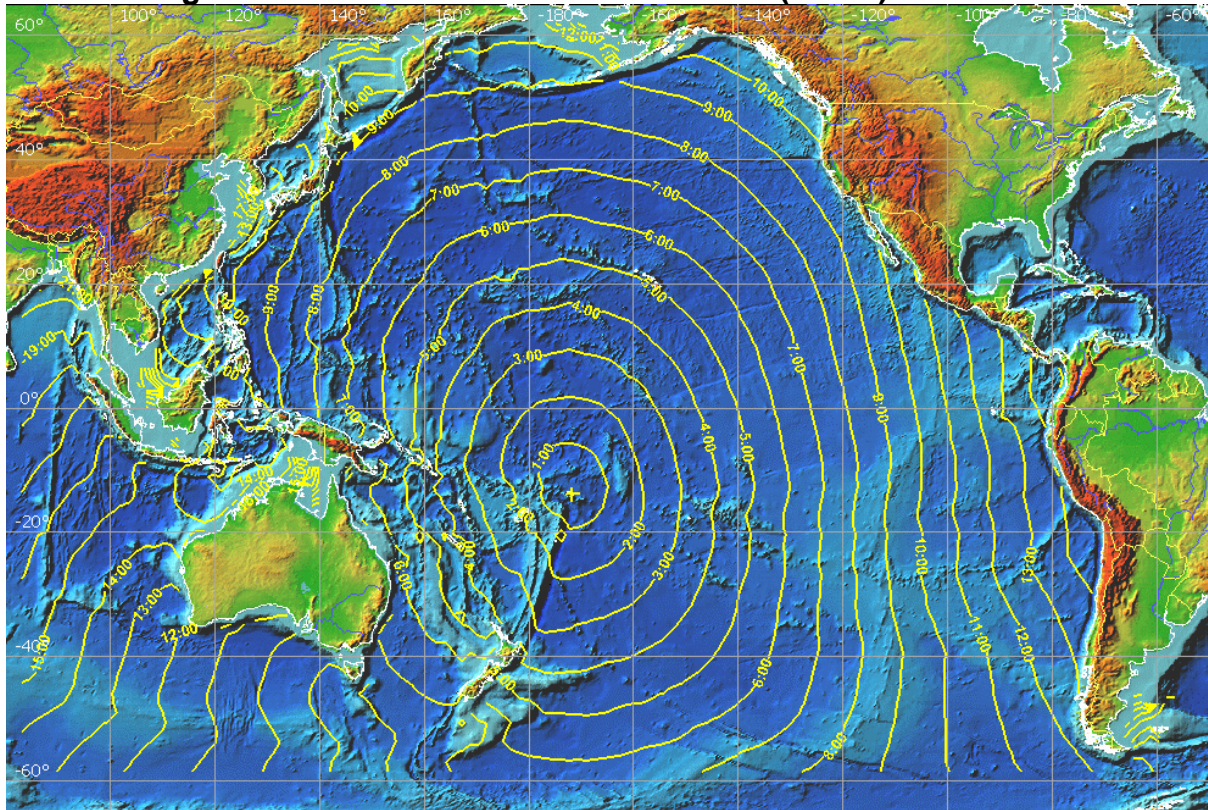
Figure 13. Inverse Tsunami Travel Times (hours) for Samoa.
