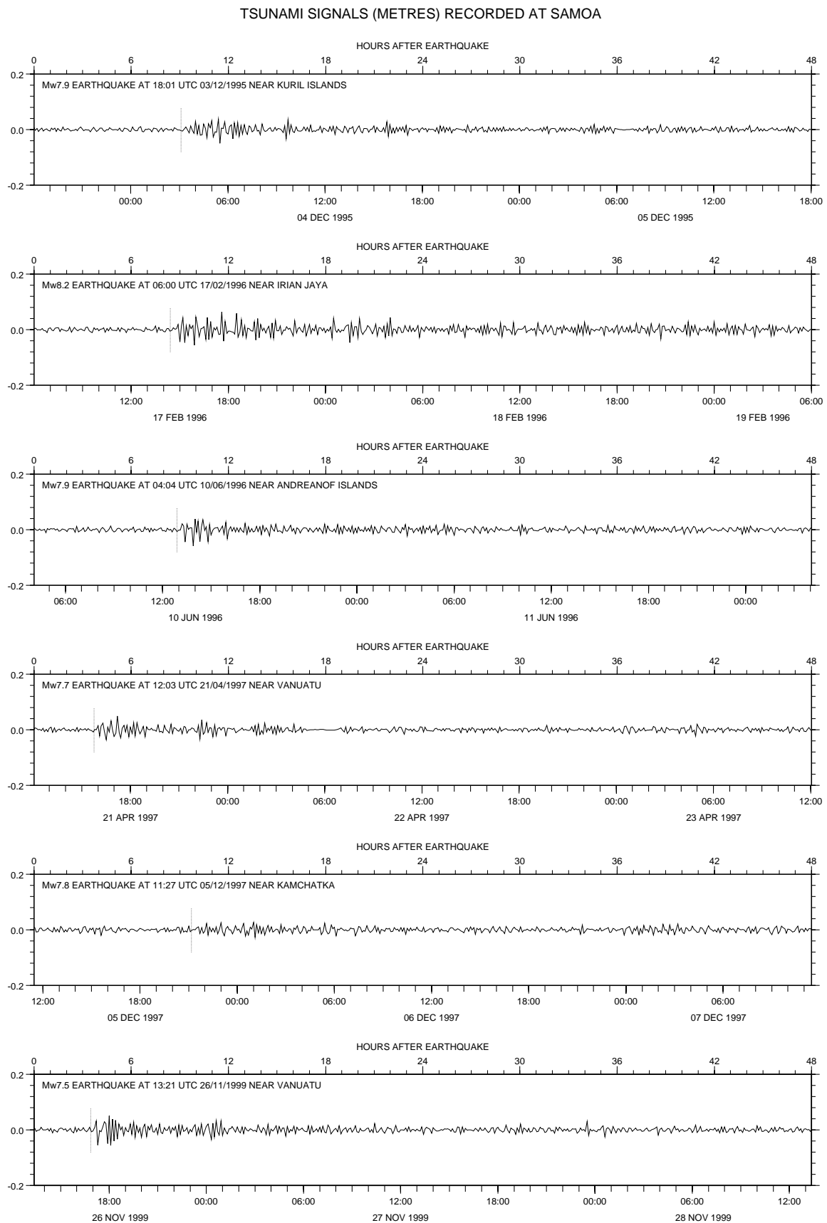
Figure 14b. Tsunami signals (m) recorded by the SEAFRAME at Apia, Samoa since installation.
