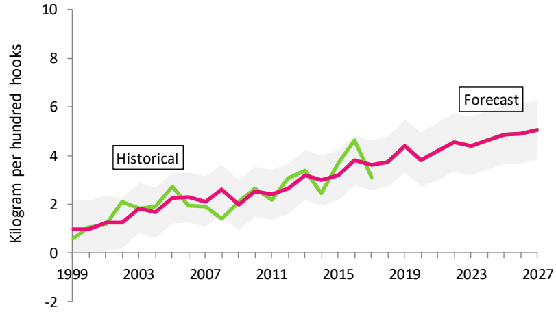
Figure 36: Projections of albacore CPUE in the tropical longline fishery
